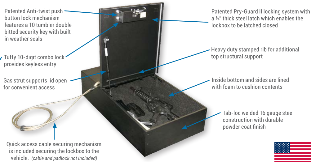
Patented Anti-twist push button lock mechanism features a 10 tumbler double bit security key.
