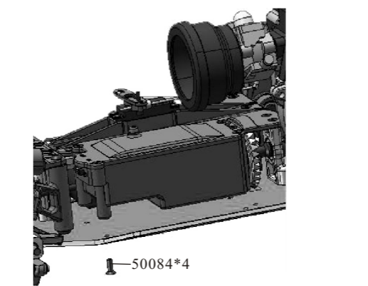
Side Guard Assembly(R/L)
