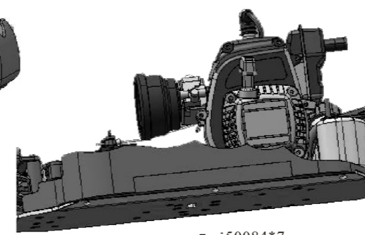
Side Guard Assembly(R/L)
