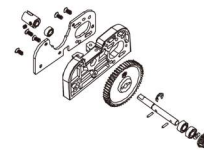
BS213-029A Spur Gear Unit (steel)
