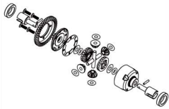
BS803-026 Diff. Gear Box Unit (steel)
