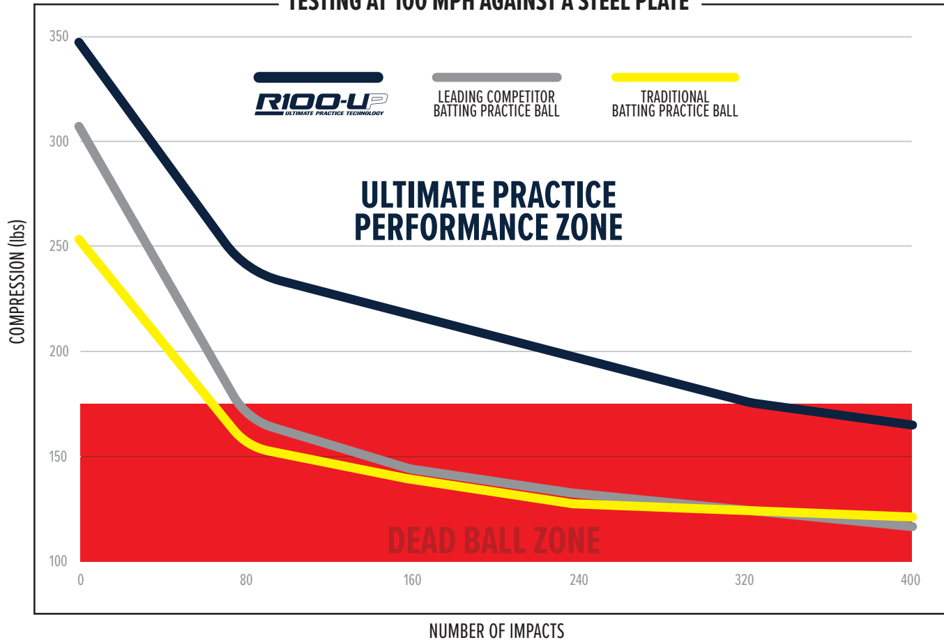
Balls tested at 100 miles per hour against a steel plate for 400 impacts. Compression measured after every 80 impacts. Compression refers to the pounds of force (lbs) necessary to compress the ball ¼ inch.
