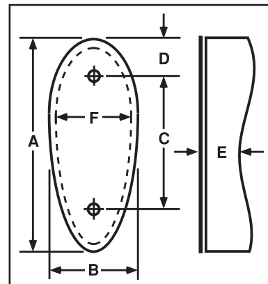
Pad Dimensions
