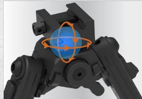
Tension Adjustable 360° Panning and 13° Tilt Forward, Rearward, Left, and Right
