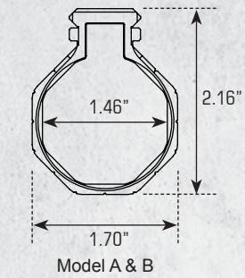
Low Profile Keymod Rail Panel Covers [Also Refer to P. 153]
