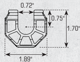
M-LOK® MTU039SSM KEYMOD MTU039SSK M-LOK® MTU043SSM KEYMOD MTU043SSK MR556 15" Rail G3 12" Rail
