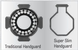
Traditional Handguard Super Slim Handguard Super Slim Design for Comfort and Weight Reduction
